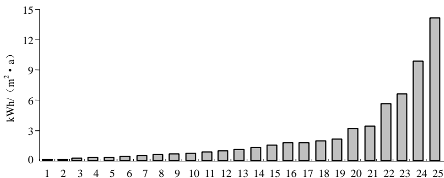
Figure 5-12 Measured air-conditioning electricity consumption per household for certain residential buildings in Beijing
