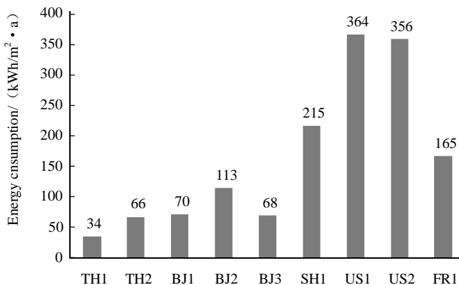
Figure 5-13 Comparison for office building energy consumption in different countries
